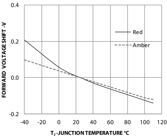
Figure 11 Forward Voltage shift vs. Junction Temperature
