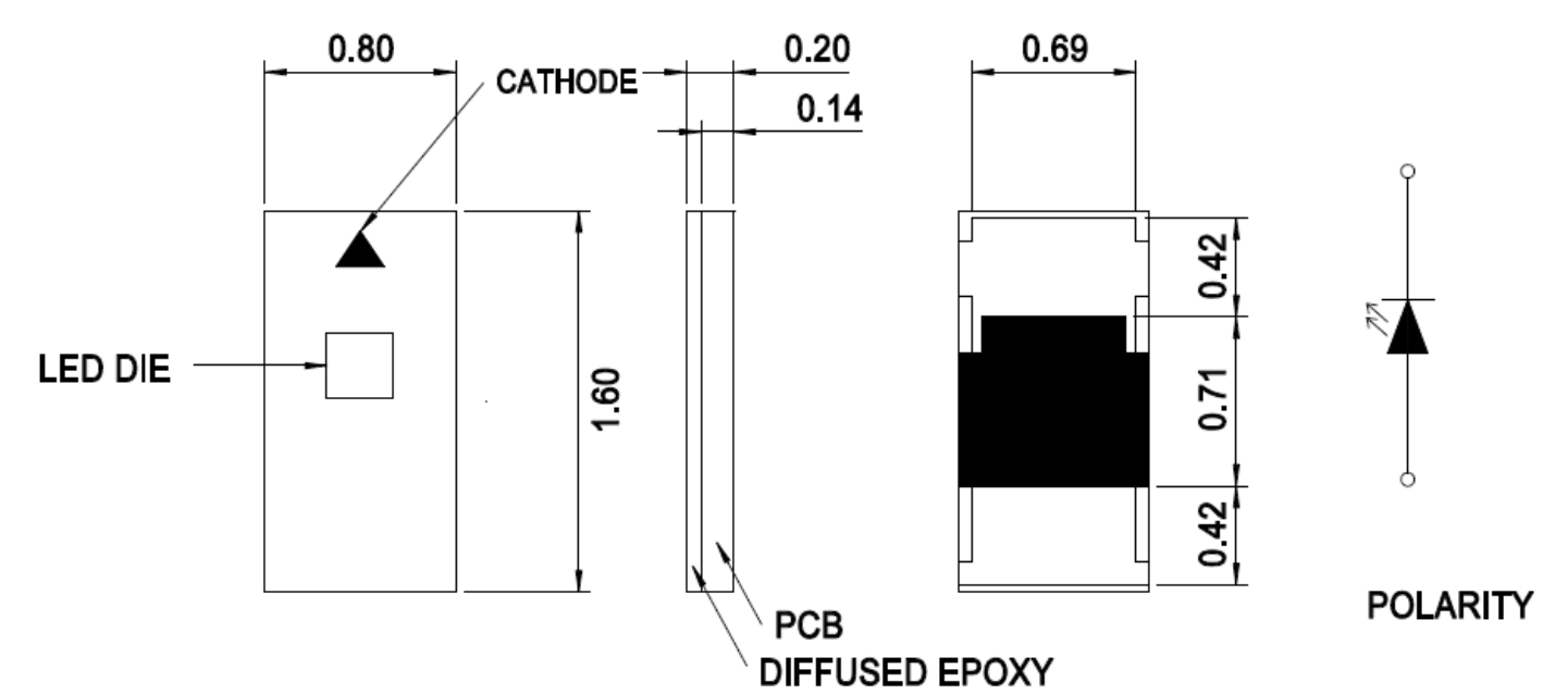
Figure 1: Package Dimensions
