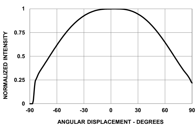
Figure 5: Radiation Pattern
