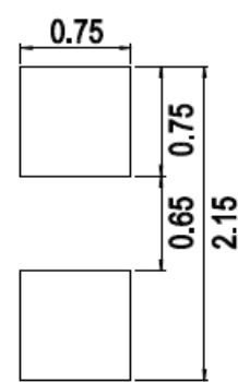
Figure 7: Recommended Soldering Land Pattern
