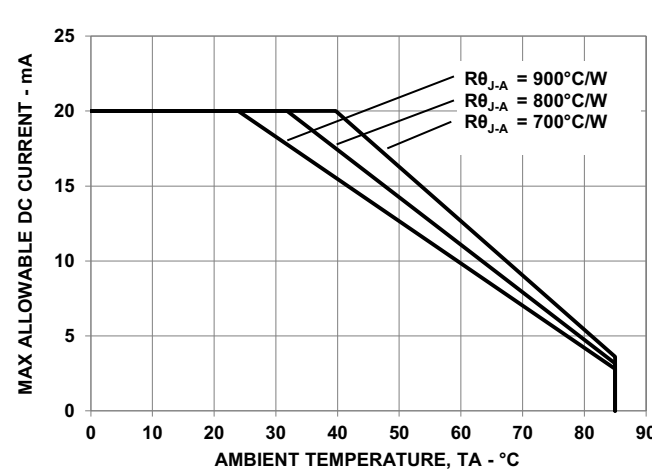
Figure 4: Derating Curve
