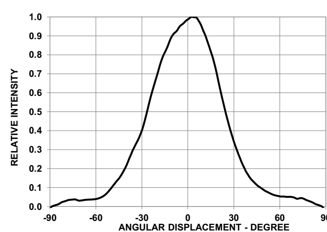
Figure 6: Radiation Pattern
