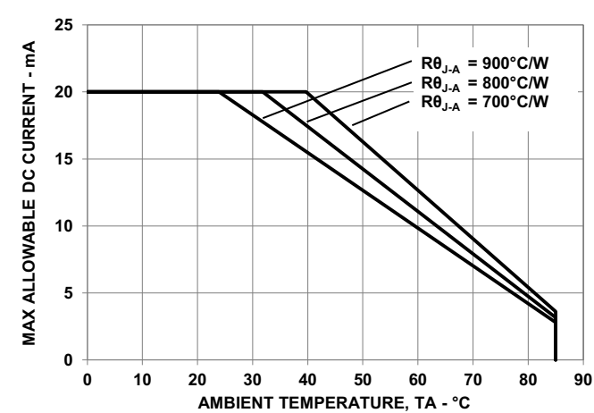
Figure 4: Derating Curve
