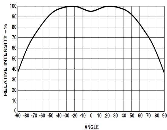
Figure 5: Radiation Pattern
