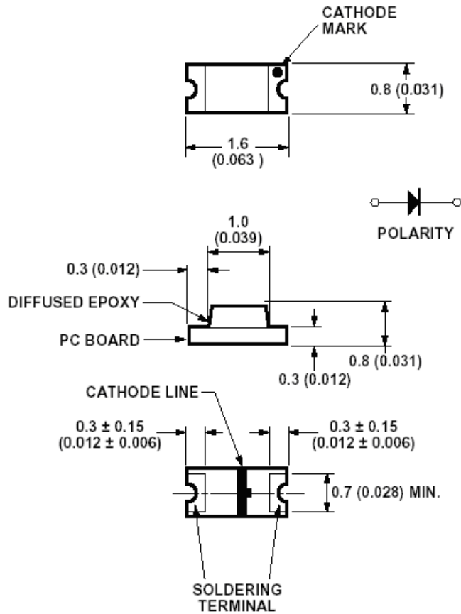
Figure 1: Package Dimensions
