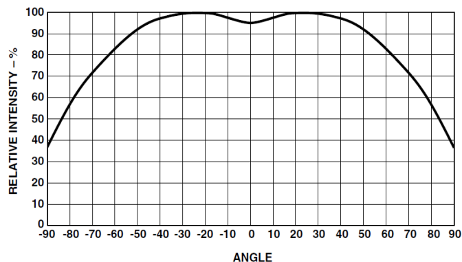
Figure 5: Radiation Pattern
