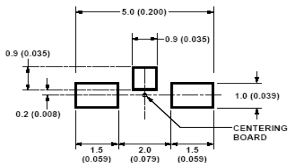
Figure 7: Recommended Soldering Land Pattern
