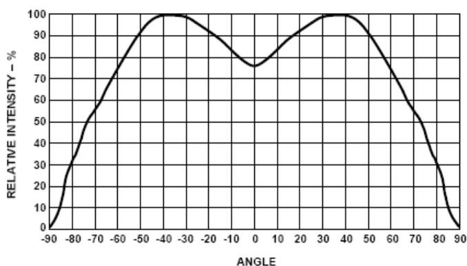
Figure 5: Radiation Pattern
