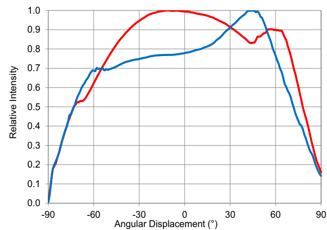
Figure 4: Radiation Pattern
