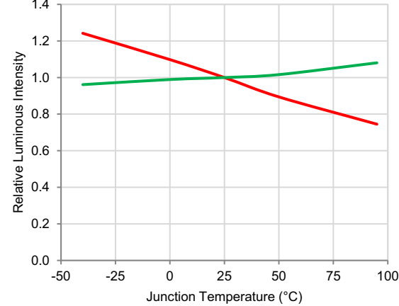
Figure 5: Relative Luminous Intensity vs. Junction Temperature
