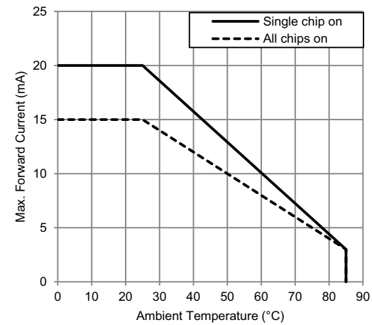
Figure 9: Derating Curve
