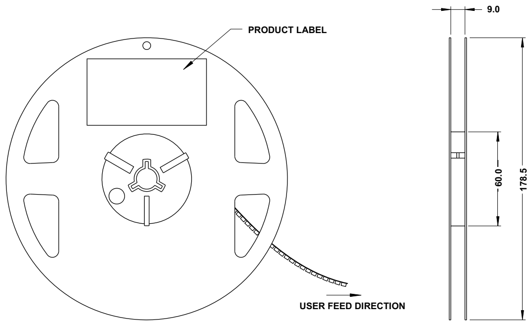
Figure 11: Reel Dimensions
