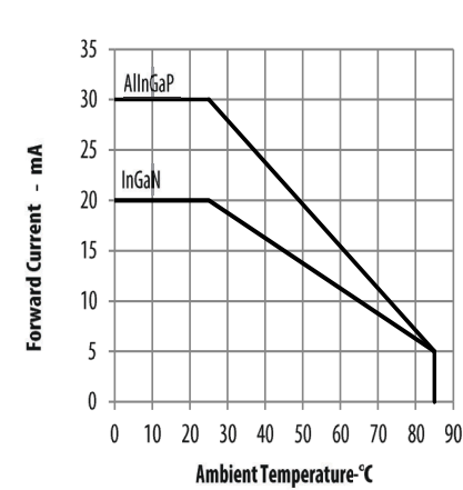
Figure 8: Derating Curve
