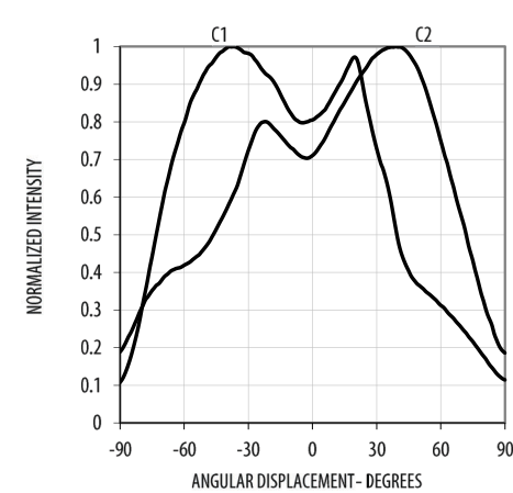
Figure 6: Radiation Pattern, Manufacturing Site 1
