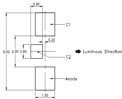
Figure 9: Recommended Solder Pad
