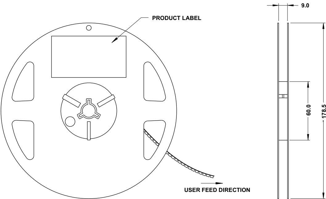
Figure 11: Reel Dimensions
