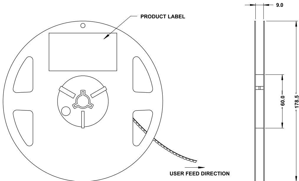
Figure 11: Reel Dimensions
