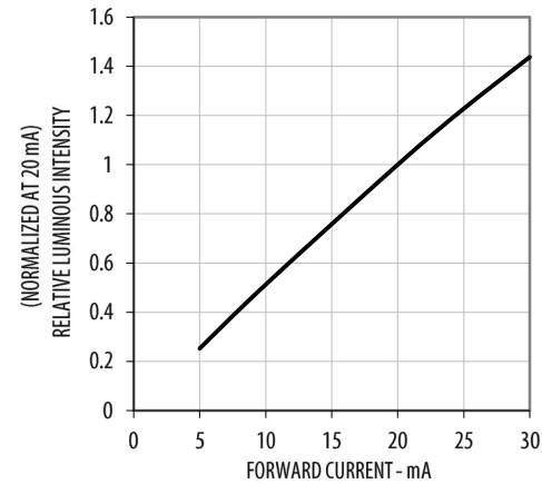
Figure 5: Relative Intensity vs. Forward Current
