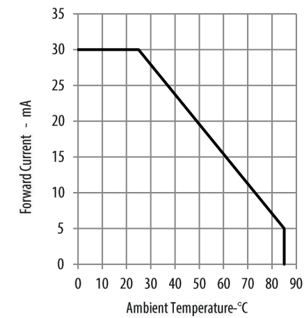
Figure 8: Derating Curve
