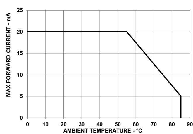
Figure 5: Derating Curve
