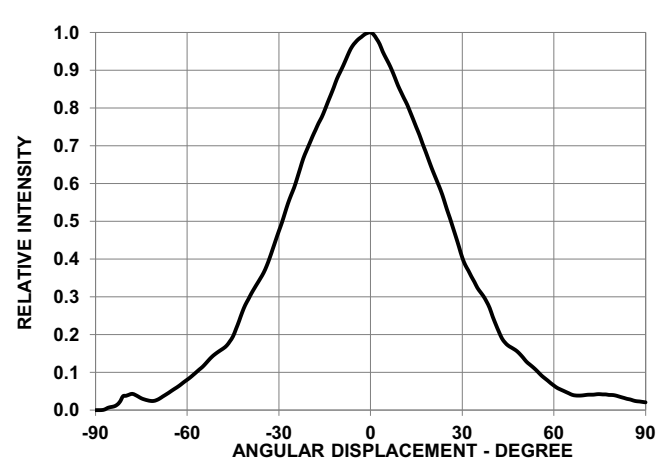
Figure 4: Radiation Pattern
