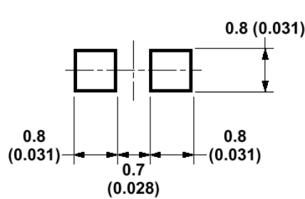
Figure 6: Recommended Soldering Land Pattern
