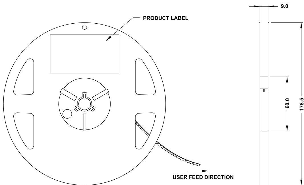
Figure 8: Reel Dimensions
