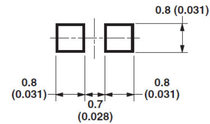
Figure 5: Recommended Soldering Land Pattern
