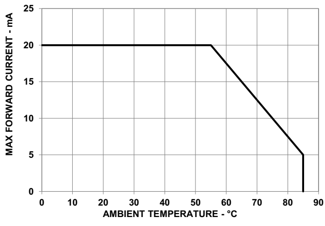
Figure 4: Derating Curve
