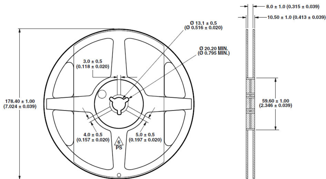
Figure 8: Reel Dimensions
