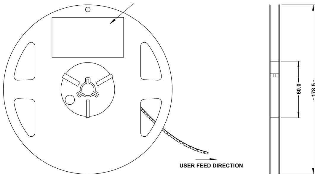
Figure 9: Reel Dimensions
