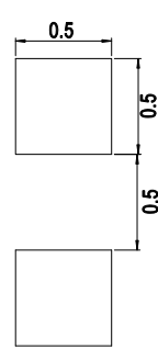
Figure 7: Recommended Soldering Land Pattern
