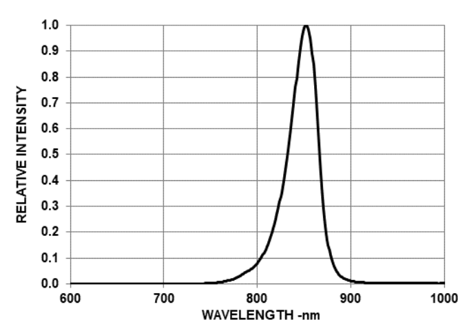
Figure 6: Spectral Distribution
