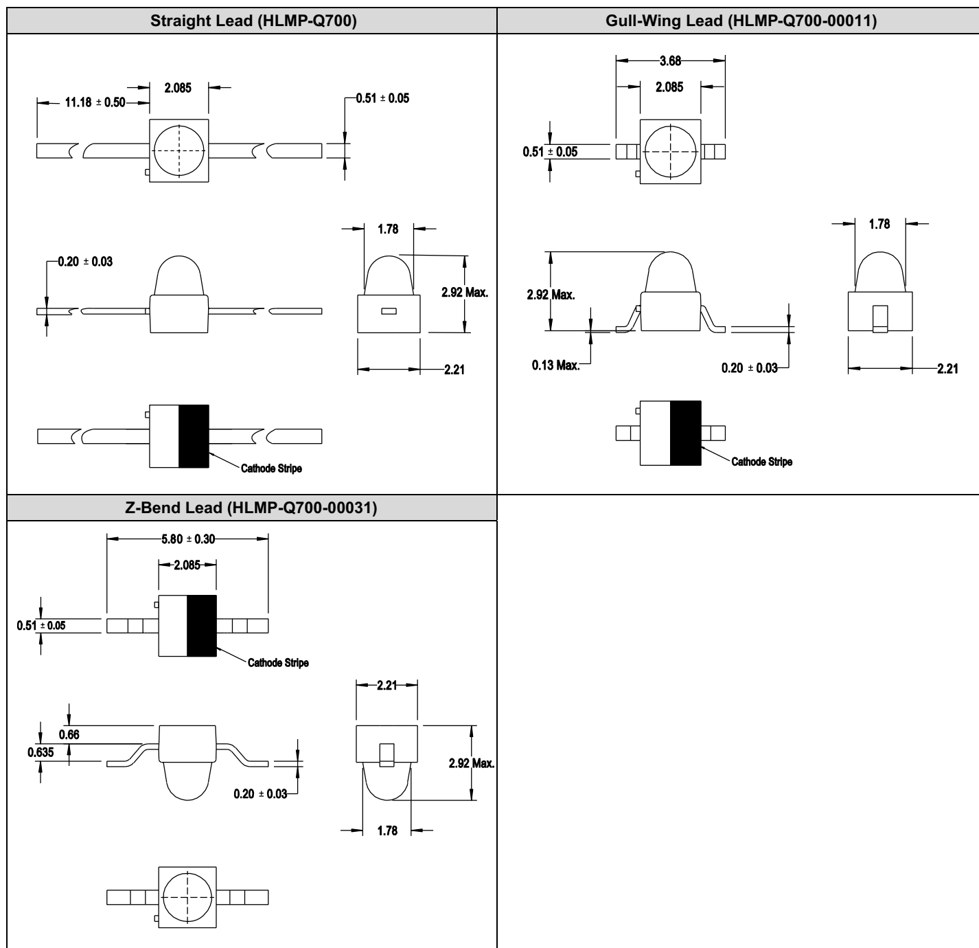
Figure 1: Package Drawing
