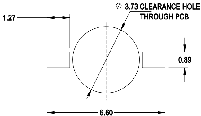
Figure 10: Recommended Soldering Land Pattern for Z-Bend Lead
