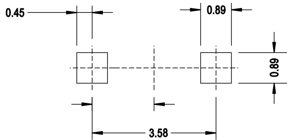
Figure 9: Recommended Soldering Land Pattern for Gull-Wing Lead
