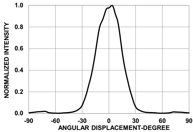
Figure 8: Radiation Pattern
