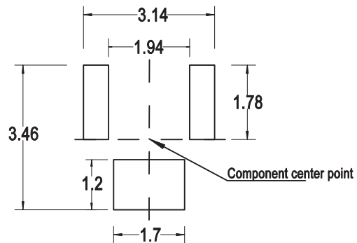
Figure 10: Recommended Soldering Land Pattern
