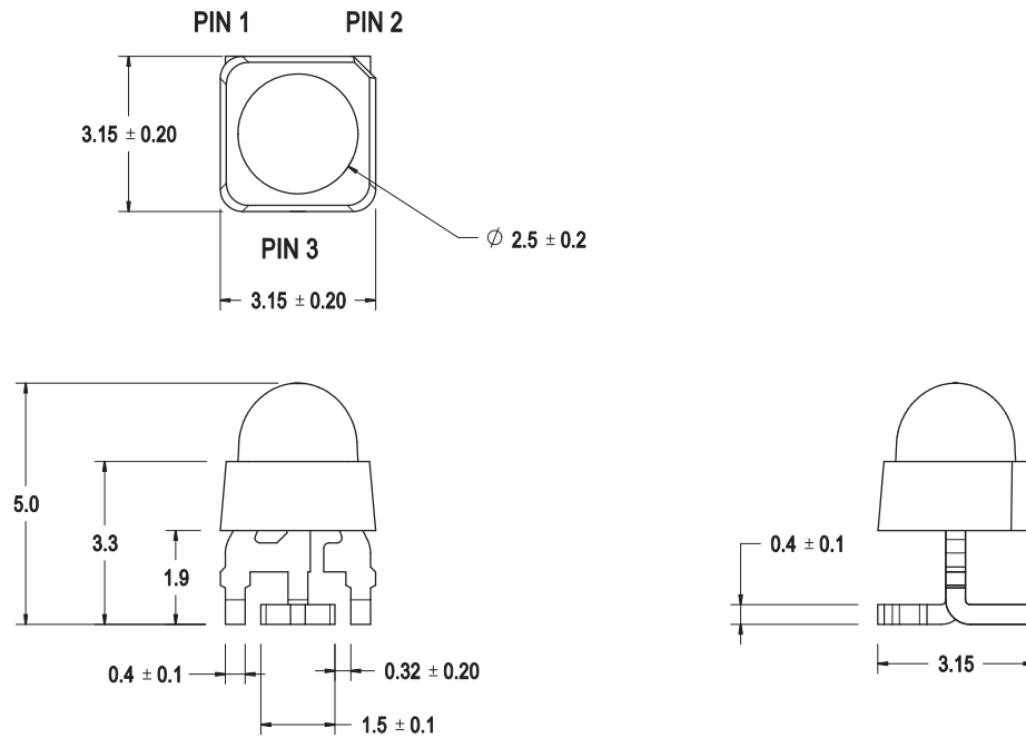
Figure 1: Package Drawing
