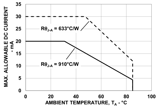
Figure 9: Maximum Forward Current vs. Ambient Temperature. Derate based on T_{J\text{ MAX}} = 110^{\circ}\text{C} (Green), T_{J\text{ MAX}} = 100^{\circ}\text{C} (Blue).
