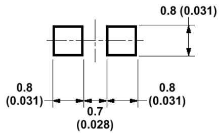
Figure 9: Recommended Soldering Land Pattern
