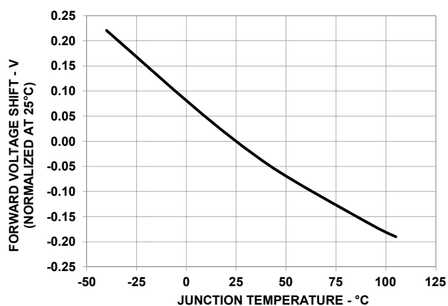
Figure 4: Forward Voltage vs. Temperature
