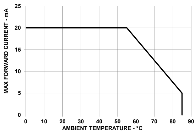
Figure 6: Derating Curve
