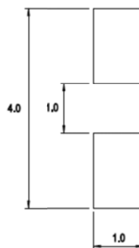
Figure 7: Recommended Soldering Land Pattern
