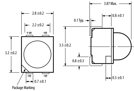
Power PLCC-4 with Lens
