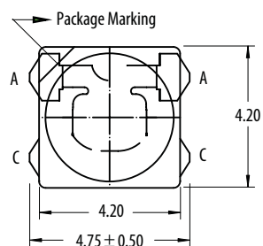
Package Drawing C
