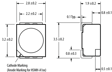
PLCC-2 Top Mount
