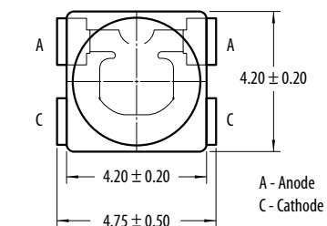
Package Drawing A
