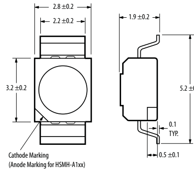
PLCC-2 Reverse Mount
