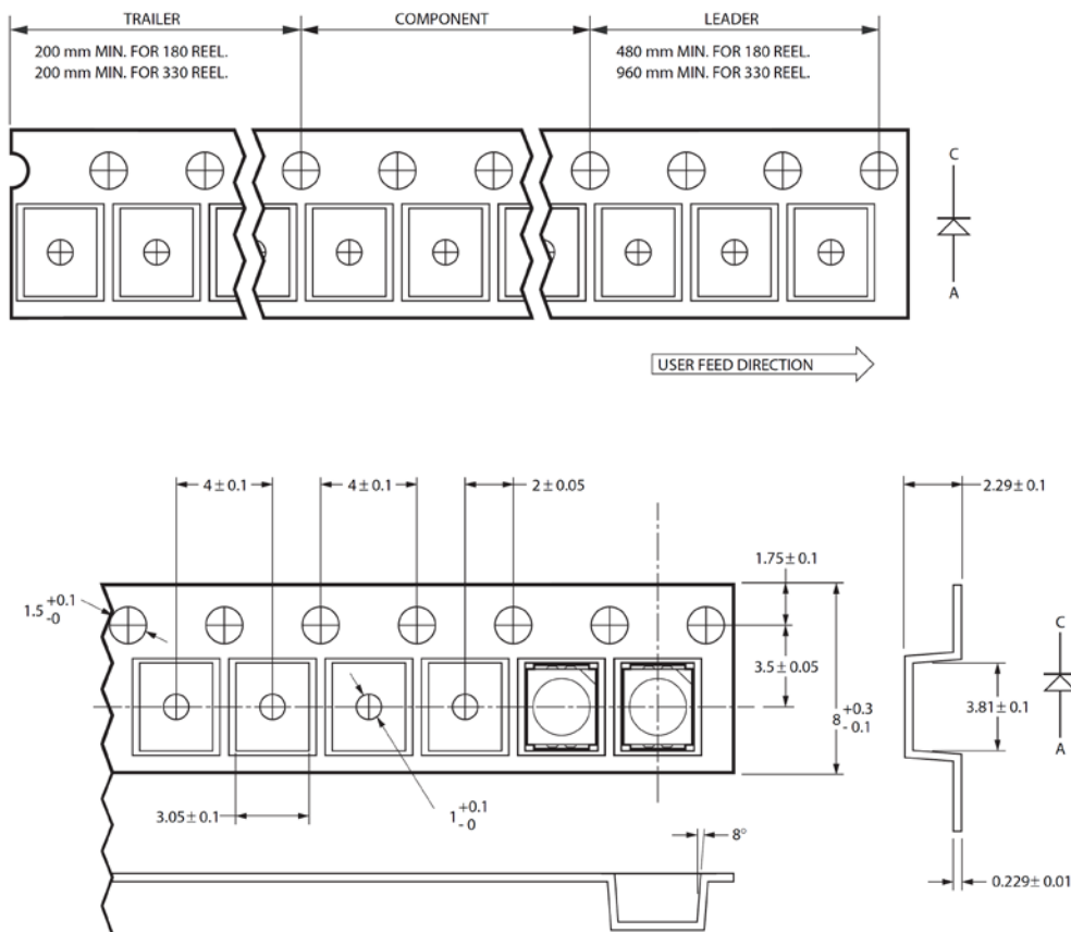
Figure 8: Carrier Tape Dimensions
