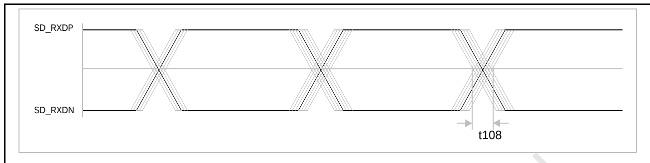
Figure 46: SGMII/SerDes Interface Input Timing
