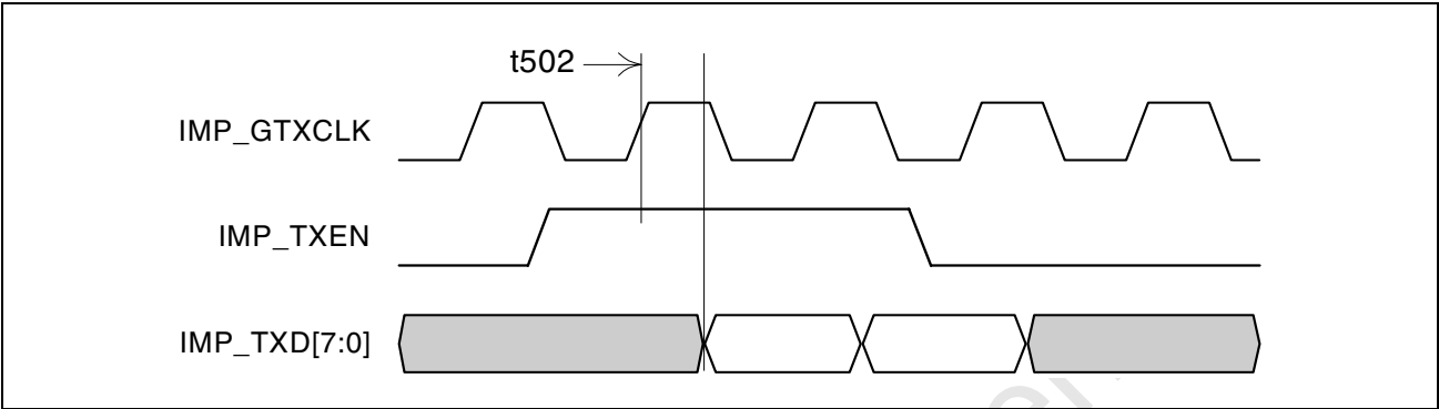
Figure 52: GMII Output Timing
