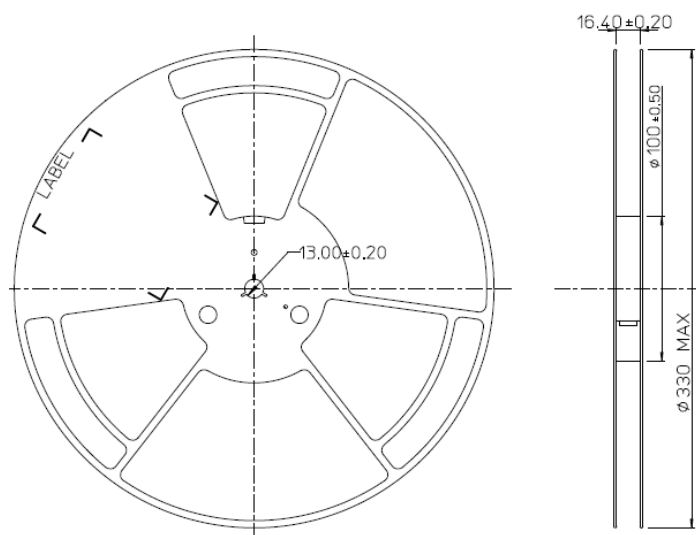
Figure 11 Reel Dimension
