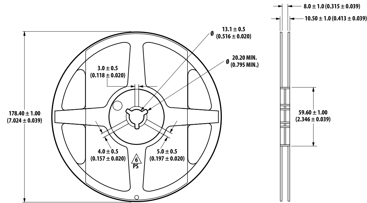
Figure 17: Reel Dimensions
