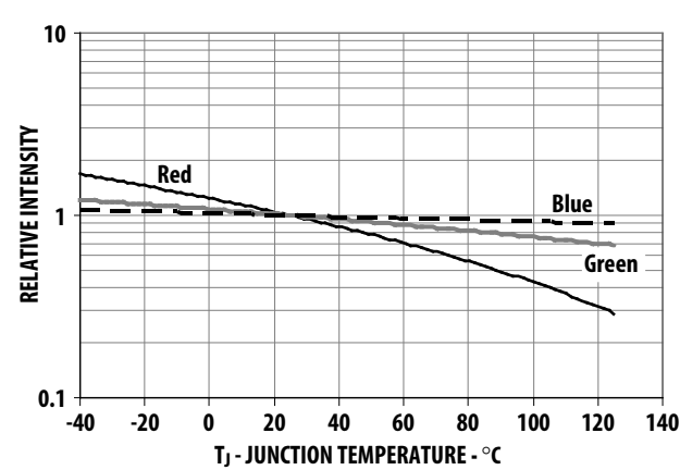
Figure 5: Relative Luminous Intensity vs. Junction Temperature
