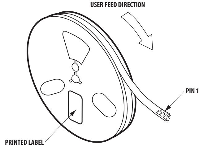
Figure 14: Reeling Orientation
