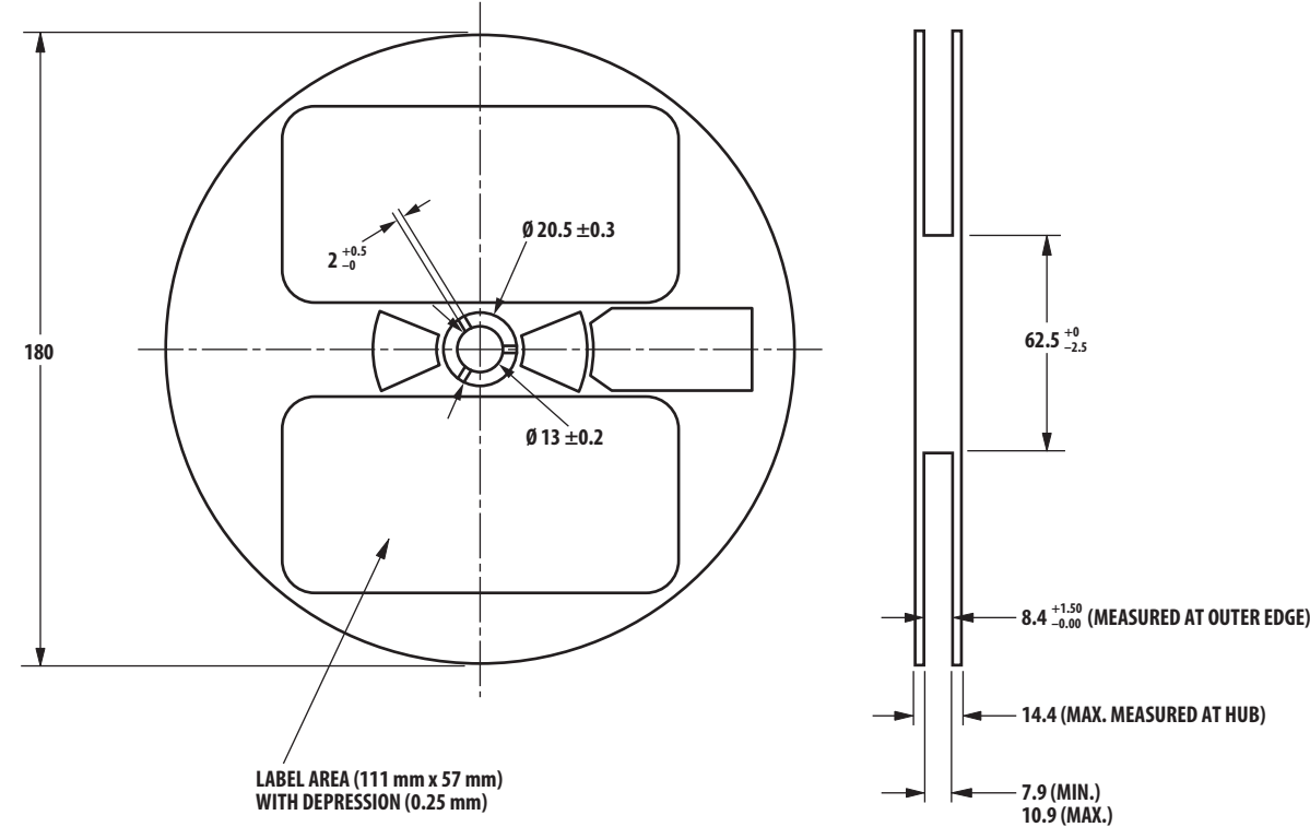
Figure 14: Reeling Orientation
