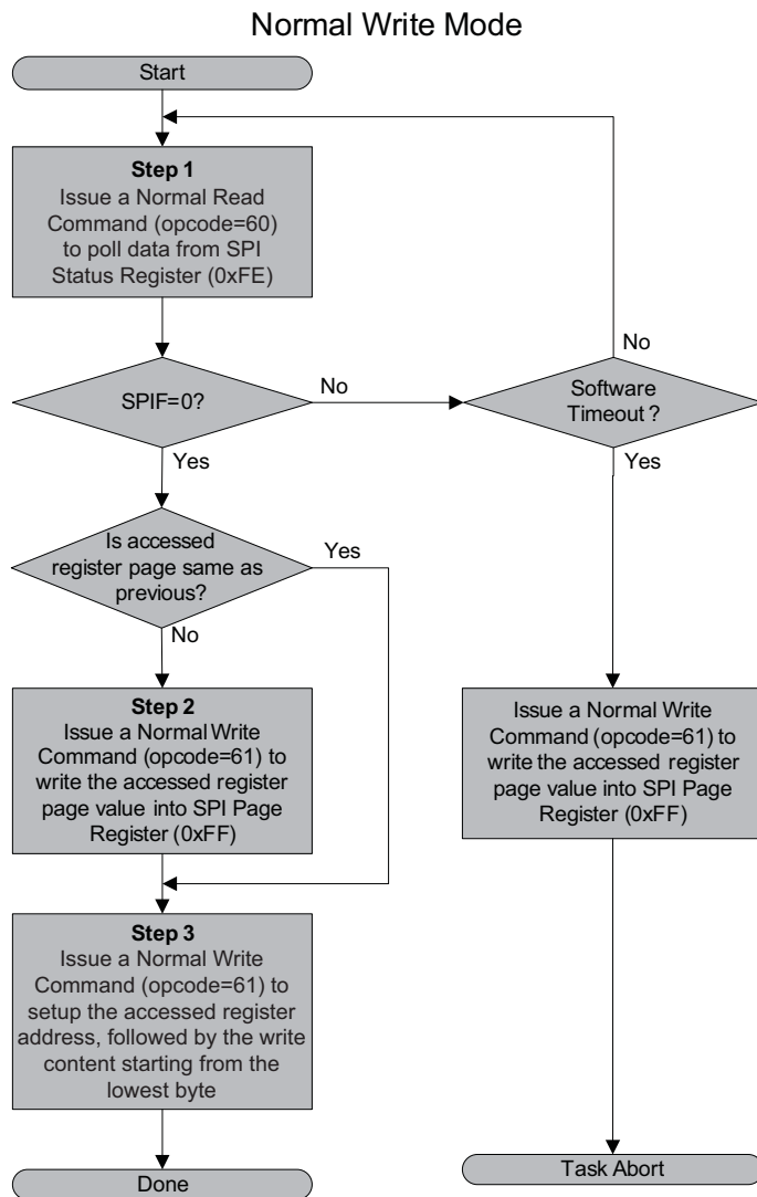
Figure 28: Normal Write Operation
