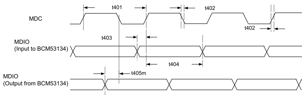
Figure 54: MDC/MDIO Timing (Master Mode)
