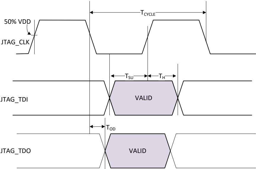
Figure 57: JTAG Interface
