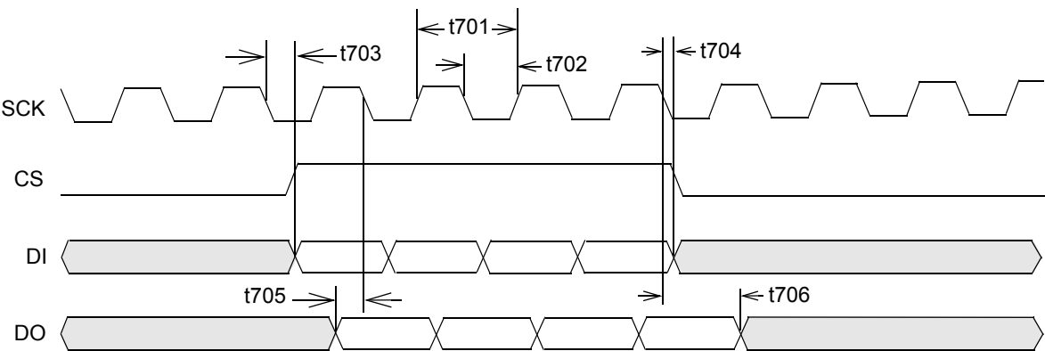
Figure 58: EEPROM Timing
