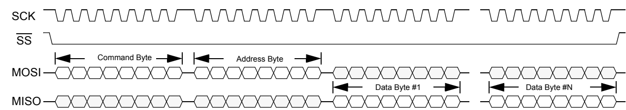
Figure 15: SPI Serial Interface Read Operation
