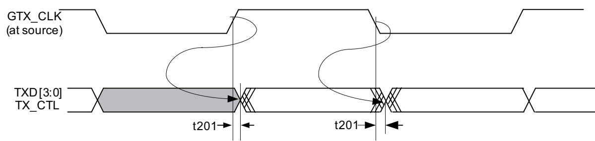
Figure 49: RGMII Output Timing (Normal Mode)
