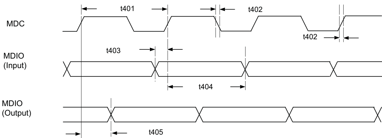
Figure 53: MDC/MDIO Timing (Slave Mode)
