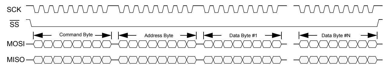
Figure 14: SPI Serial Interface Write Operation
