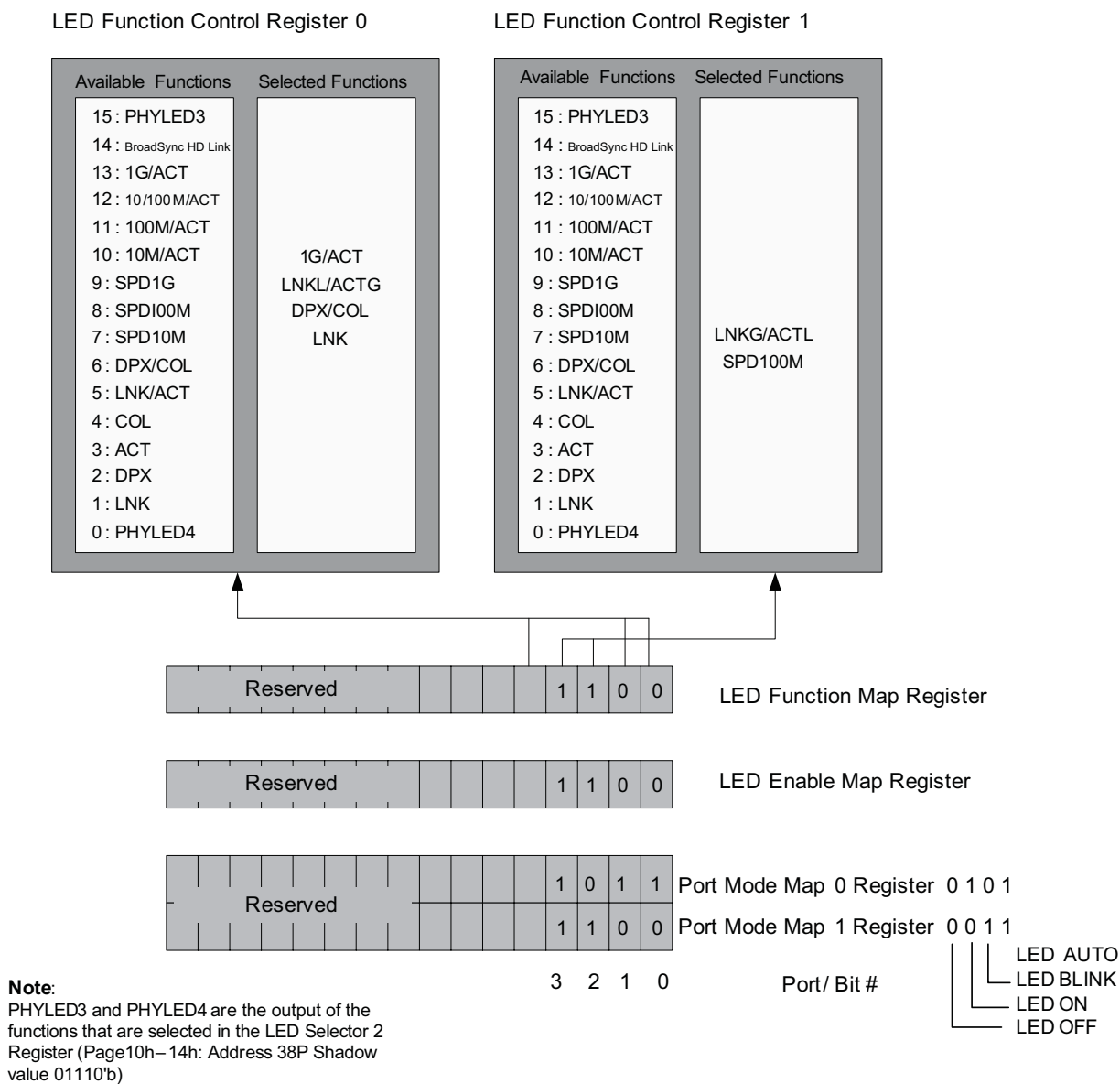
Figure 44: LED Interface Register Structure Diagram
