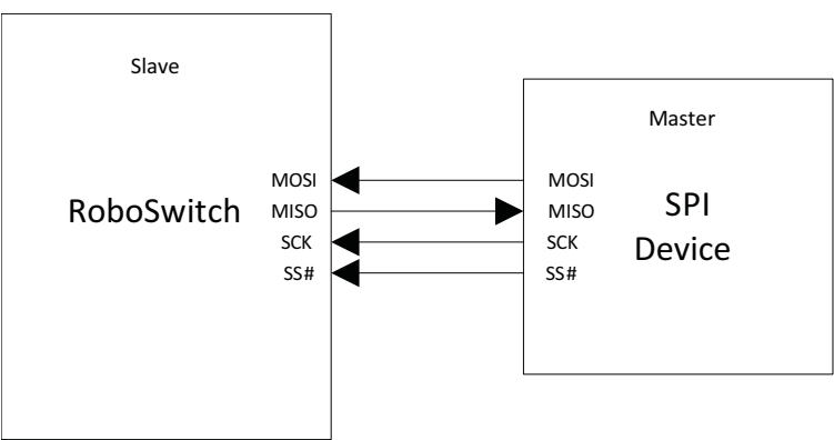
Figure 16: SPI Interface Without External PHY Device
