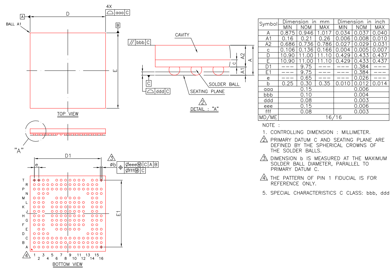
Figure 63: BCM531340 Mechanical Information
