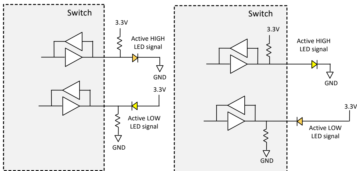
Figure 47: Dual Input Configuration/LED Output Function
