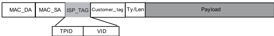
Figure 6: ISP Tag Diagram
