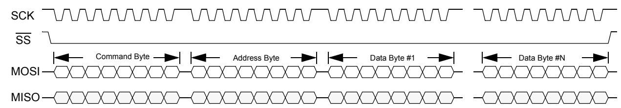
Figure 26: SPI Serial Interface Write Operation
