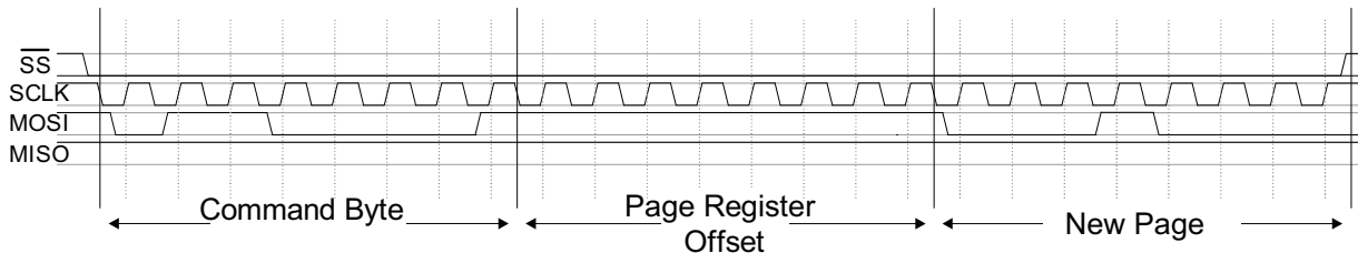
Figure 42: Normal Write to Setup the Register Page Value
