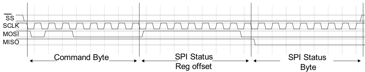
Figure 37: Normal Read Mode to Check the SPIF Bit of SPI Status Register
