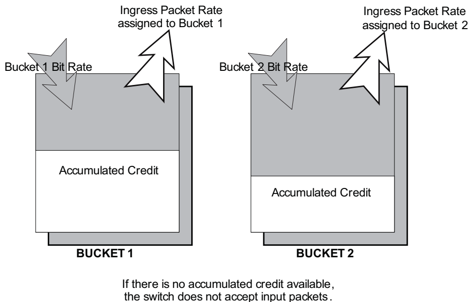
Figure 9: Bucket Flow
