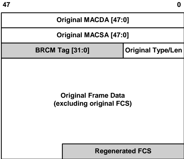
Figure 24: IMP Packet Encapsulation Format
