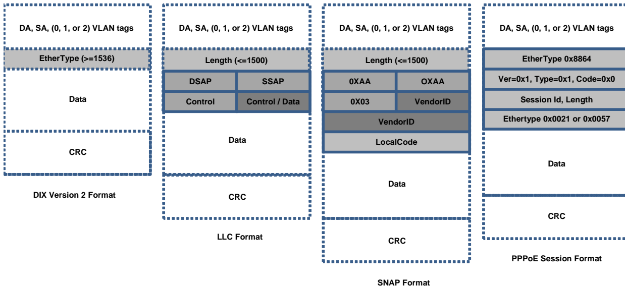
Figure 14: Ethernet Framing Structures
