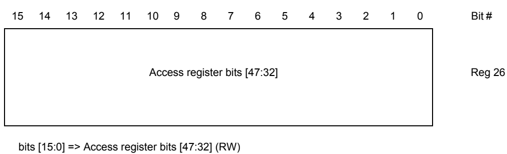
Figure 52: Pseudo-PHY MII Register 26: Access Register Bit Definition
