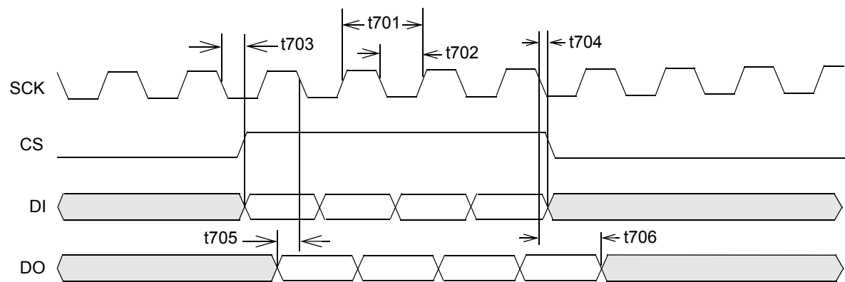
Figure 70: EEPROM Timing
