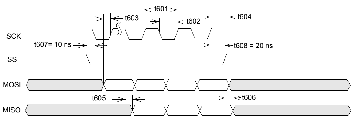
Figure 68: SPI Timings, SS Asserted During SCK High
