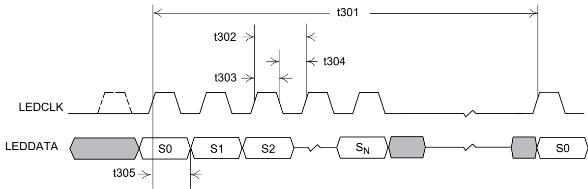
Figure 67: Serial LED Interface Timing
