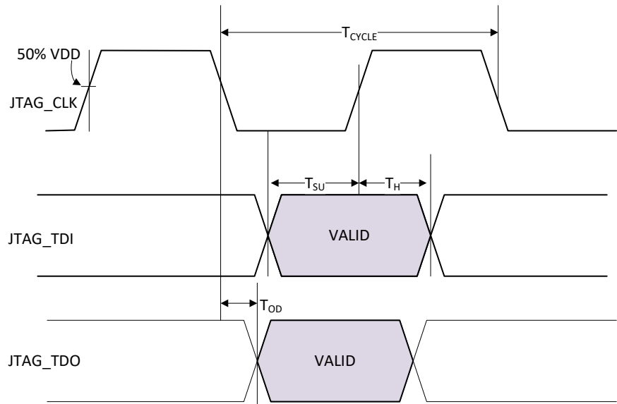
Figure 69: JTAG Interface
