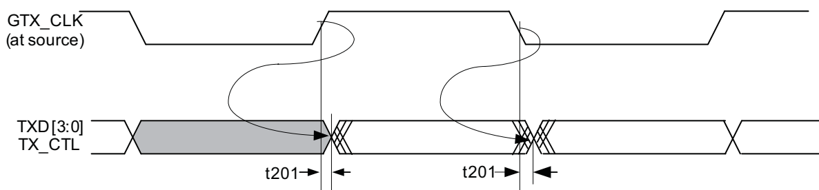
Figure 61: RGMII Output Timing (Normal Mode)
