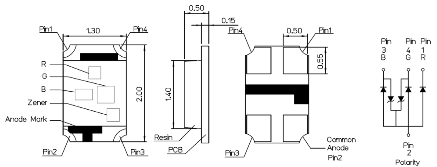
Figure 1: Package Dimensions
