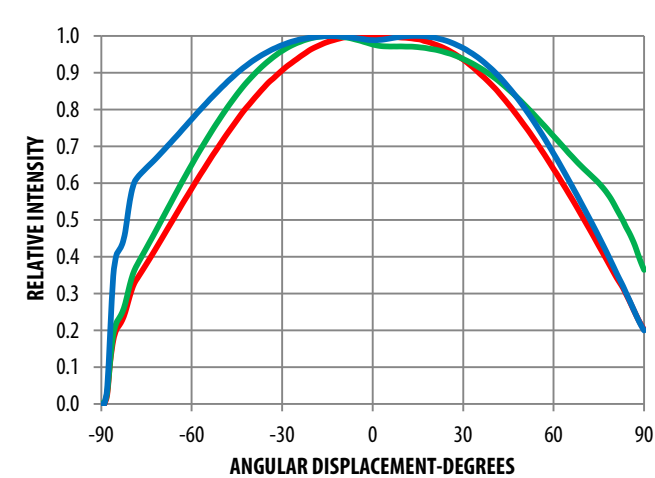
Figure 5: Radiation Pattern
