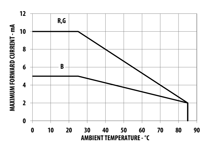
Figure 6: Derating Curve
