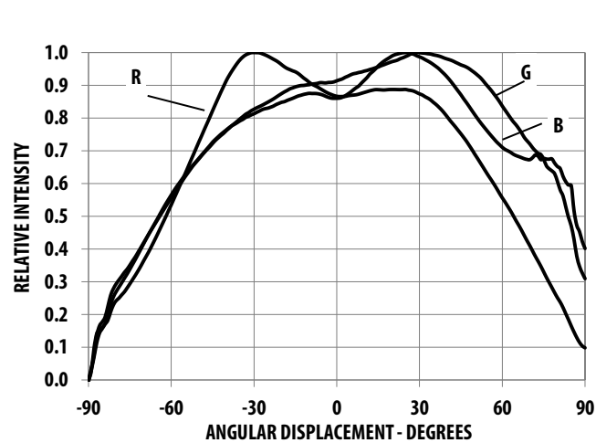
Figure 5: Radiation Pattern
