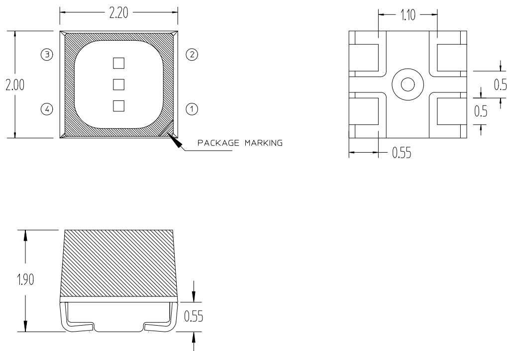
Figure 1: Package Drawing
