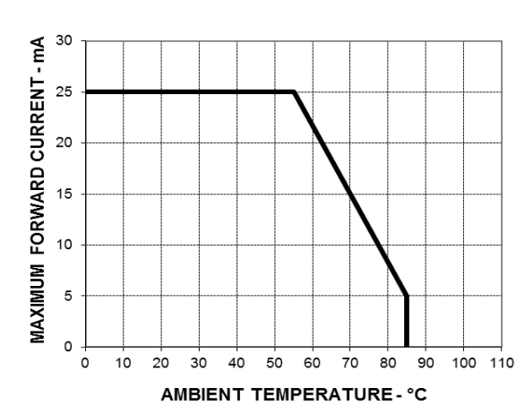
Figure 10: Forward Current vs. Temperature
