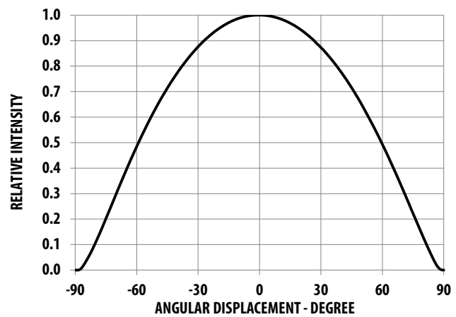
Figure 6: Radiation Pattern
