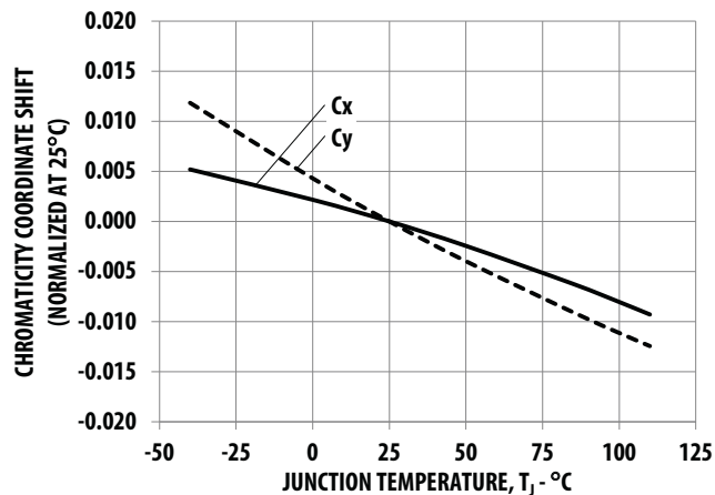
Figure 14: Chromaticity Coordinate Shift vs. Junction Temperature for 6500K
