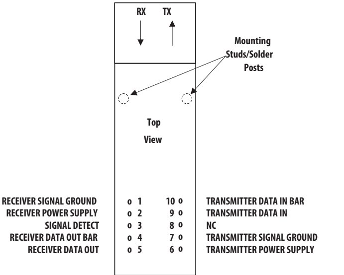
Figure 1 Pin Out Diagram
