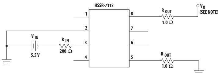
Figure 20 Burn-In Circuit
