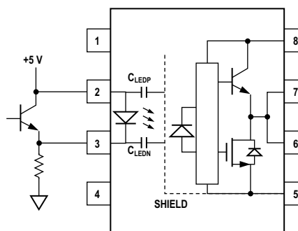
Figure 32. Recommended LED Drive Circuit for Ultra-High CMR
