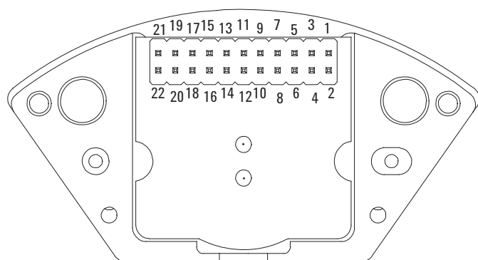
Figure 2. Pinout Configuration
