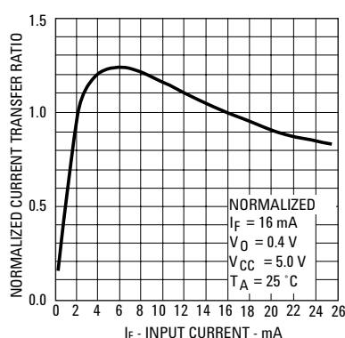
Figure 2. Current Transfer Ratio vs. Input Current.
