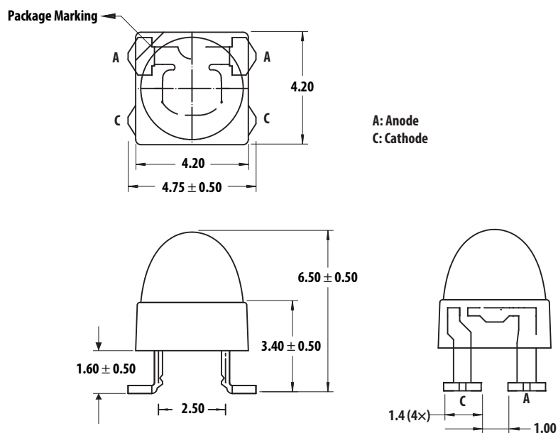
Figure 1: Package Dimensions
