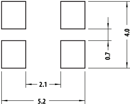
Figure 16: Recommended Soldering Land Pattern
