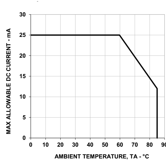
Figure 12: Maximum Forward Current vs. Ambient Temperature
