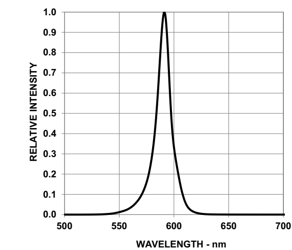
Figure 9: Relative Intensity vs. Wavelength
