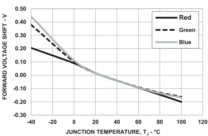
Figure 6: Forward Voltage vs. Junction Temperature
