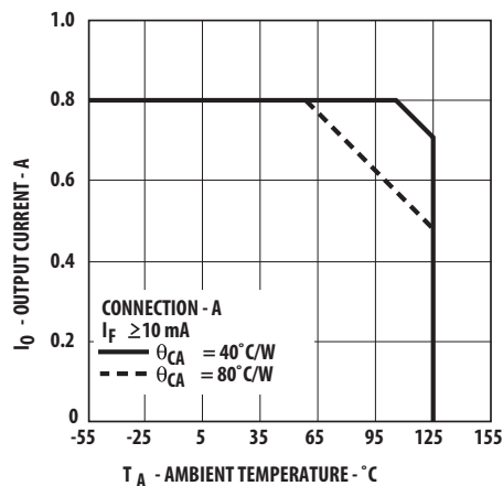
Figure 4: Output Power Rating vs. Ambient Temperature
