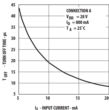
Figure 15: Typical Turn Off Time vs. Input Current
