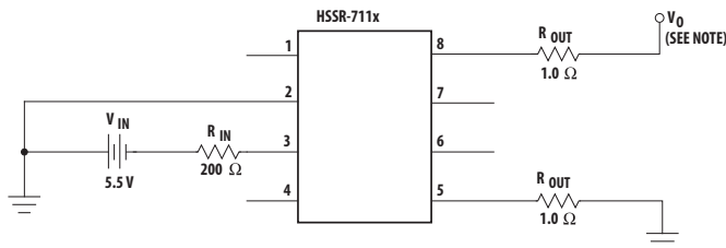
Figure 20: Burn-In Circuit
