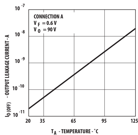
Figure 8: Typical Output Leakage Current vs. Temperature
