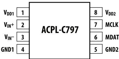
Figure 2: Pin Configuration
