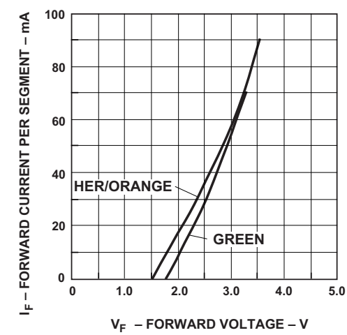
Figure 10: Forward Current vs. Forward Voltage
