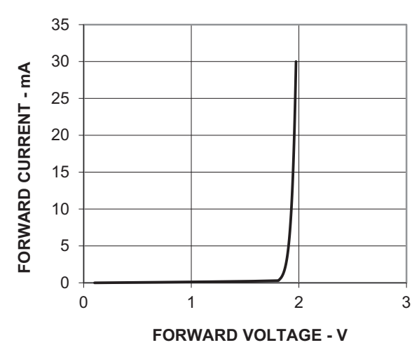
Figure 10: Forward Current vs. Forward Voltage
