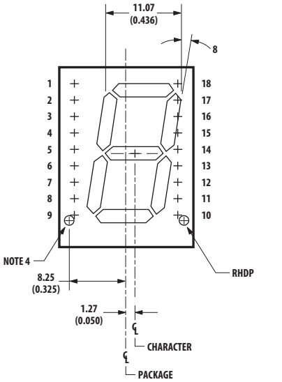
FRONT VIEW A, B
