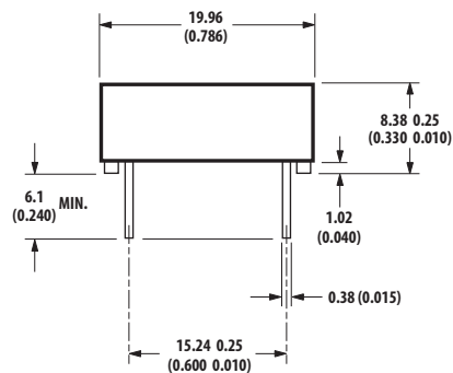
END VIEW
